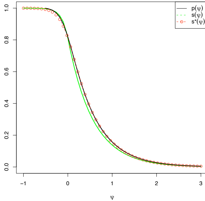
Figure 6: p -value for \psi , p(\psi) ; Bayes survivor for \psi , s(\psi) ; and linearly corrected survivor for \psi , s^*(\psi)
