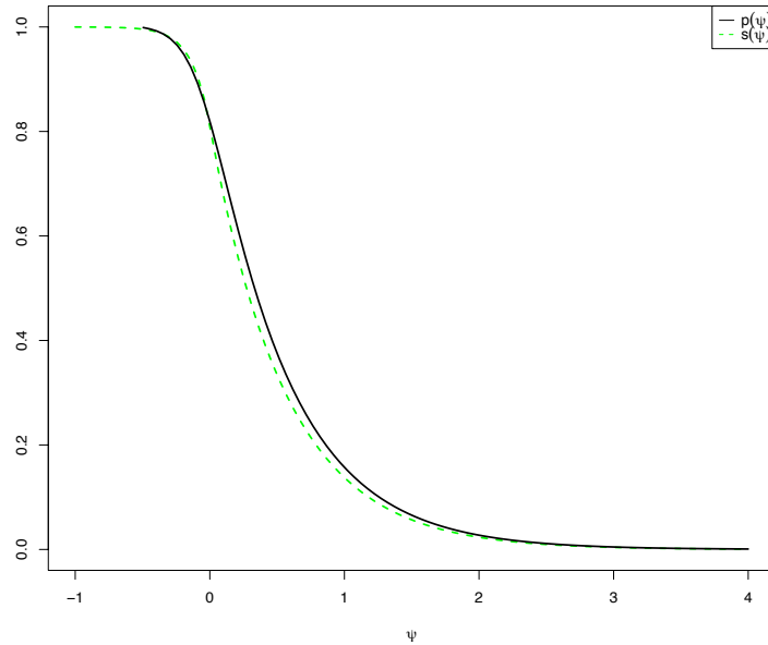
Figure 4: The posterior survival function s(\psi) for \psi = \mu/\sigma^2 for the given data; and the third order p(\psi) for the same data.
